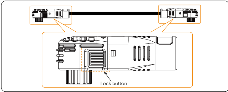
Figure 7-16 Lock button
