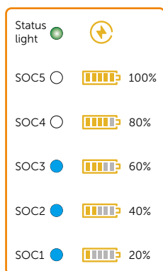
Figure 2-10 Discharging
