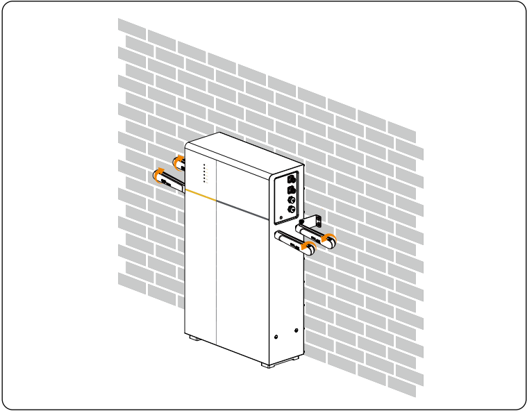
Figure 6-8 Twisting handles
