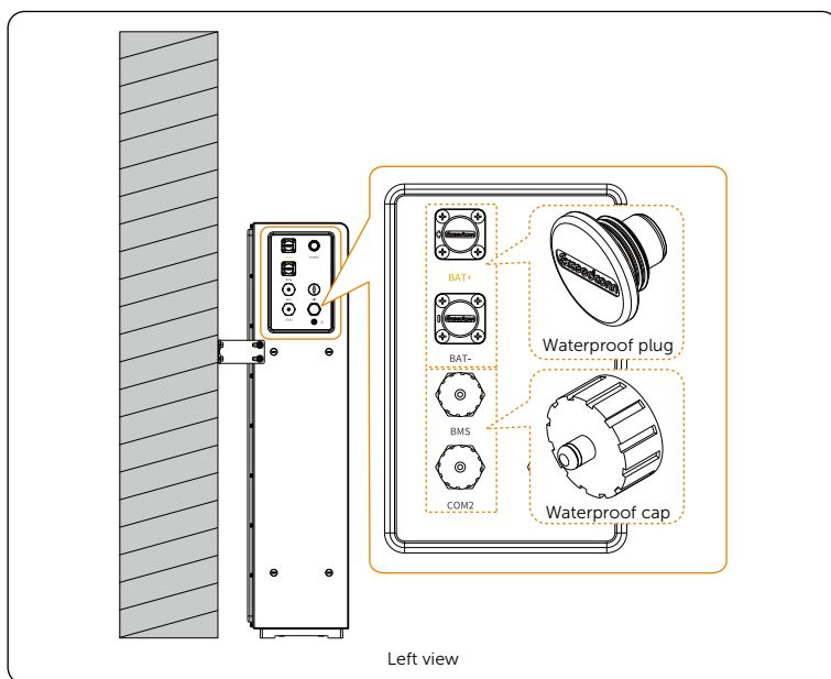
Figure 7-20 Left electrical connection area of the battery pack
