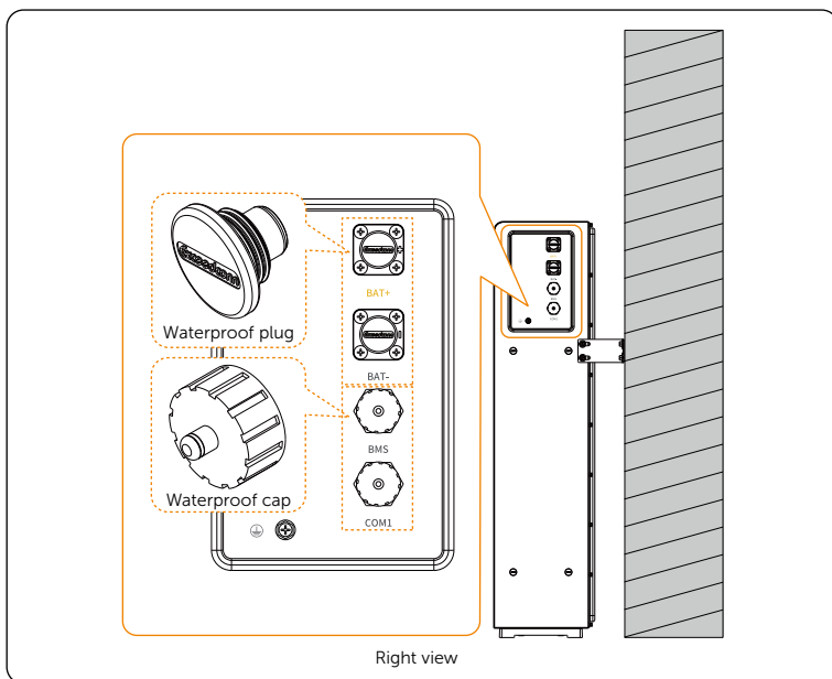
Figure 7-23 Right electrical area of the battery pack
