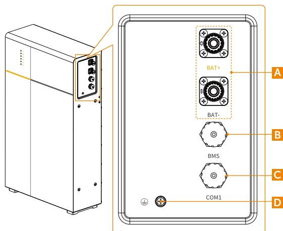
Figure 2-5 Right view
