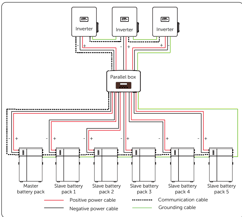
Figure 8-1 Wiring Diagram for Parallel Connection
