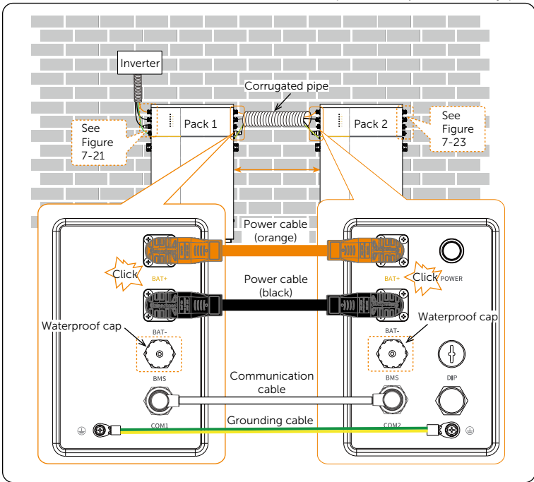
Figure 9-2 Cable connection between adjacent battery pack
