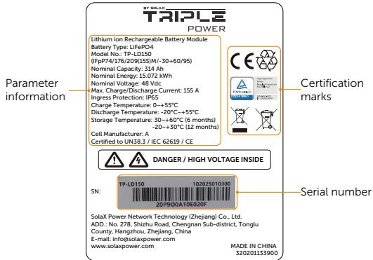
Figure 2-3 Performance label
