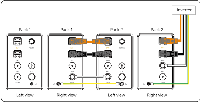
Figure 7-28 Wiring diagram
