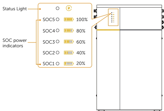
Figure 2-8 Indicators
