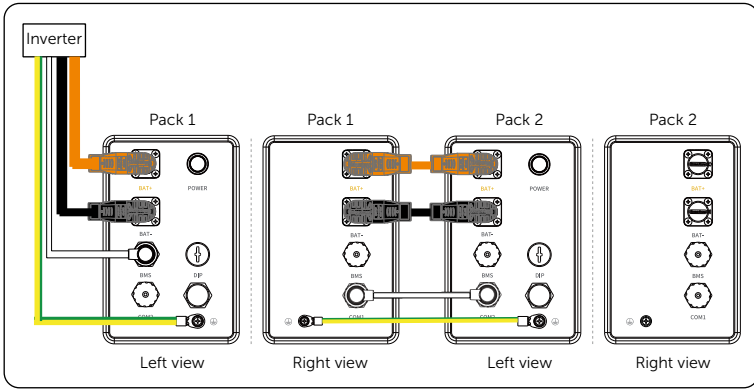
Figure 7-24 Wiring diagram
