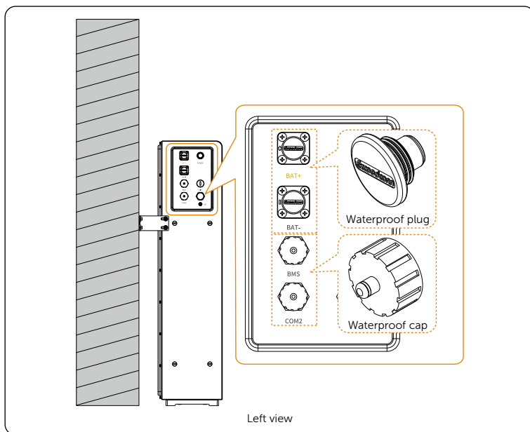
Figure 7-27 Left electrical connection area of the battery pack
