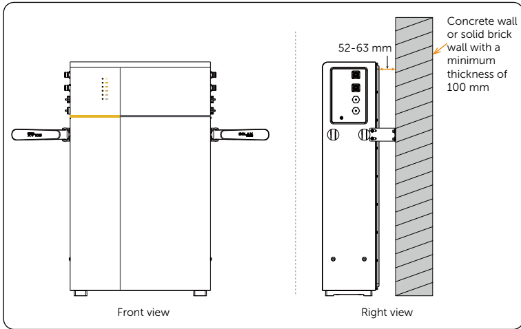
Figure 6-3 Locating the battery pack against the wall
