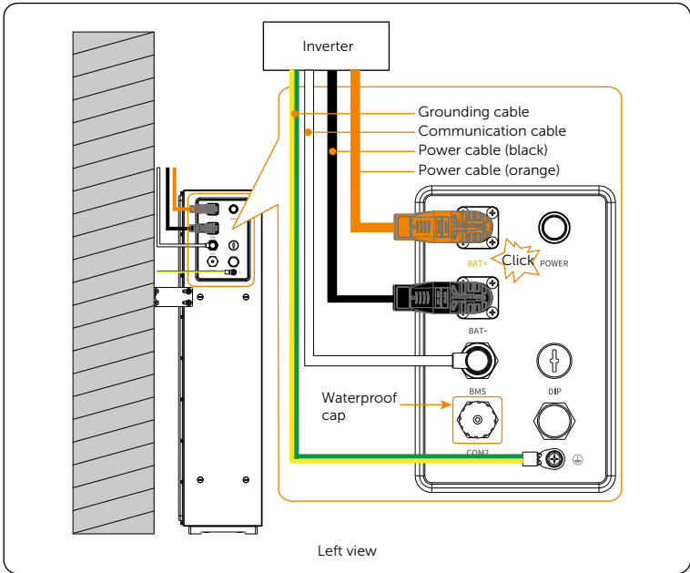
Figure 7-17 Cable connection of the left electrical connection area
