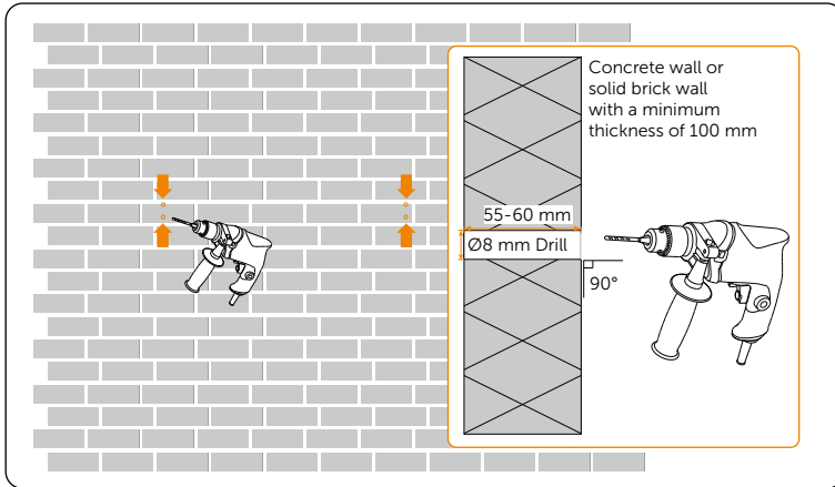
Figure 6-5 Drilling holes
