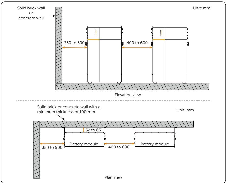
Figure 4-2 Clearance requirement
