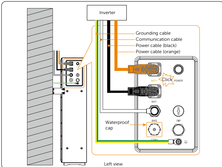
Figure 9-1 Cable connection between the master battery pack and inverter
