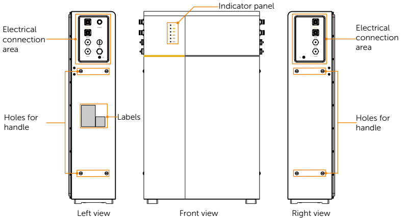
Figure 2-1 Appearance
