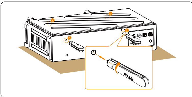
Figure 5-4 Inserting handles
