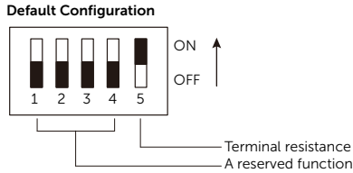
Figure 2-7 Default configuration
