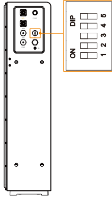
Figure 2-6 Position of DIP Switch
