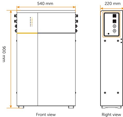
Figure 2-2 Dimension: Battery pack (TP-LD150)
