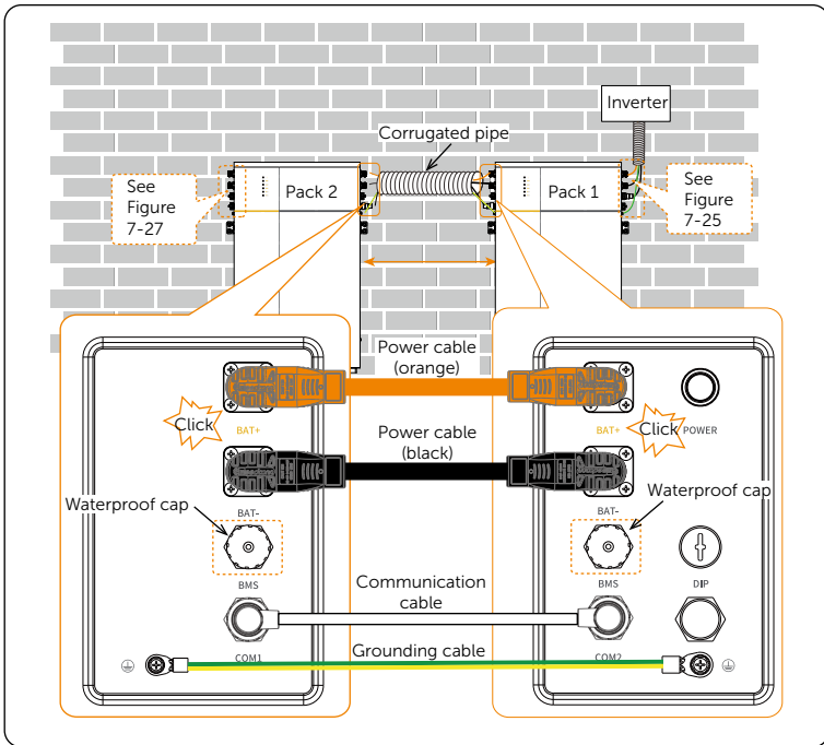
Figure 7-26 Wiring between battery packs
