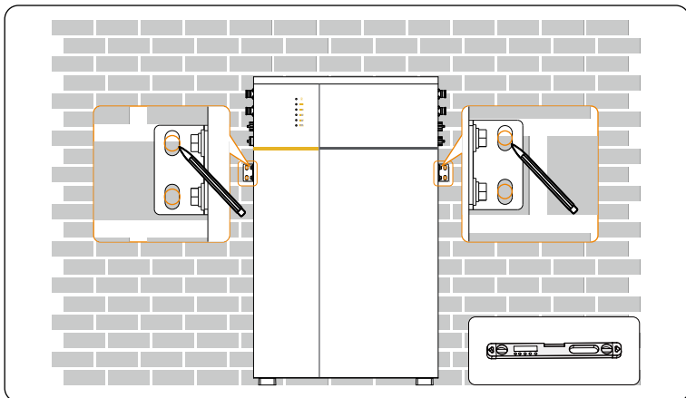
Figure 6-4 Drawing circles
