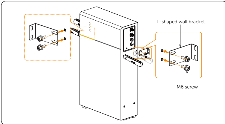
Figure 6-2 Fixing L-shaped wall bracket to the battery pack
