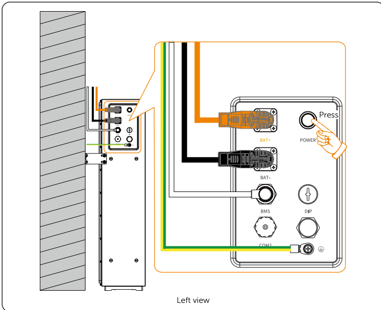
Figure 12-1 Pressing power button
