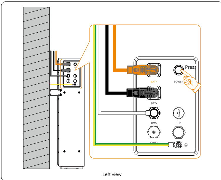
Figure 10-1 Power on/off the system
