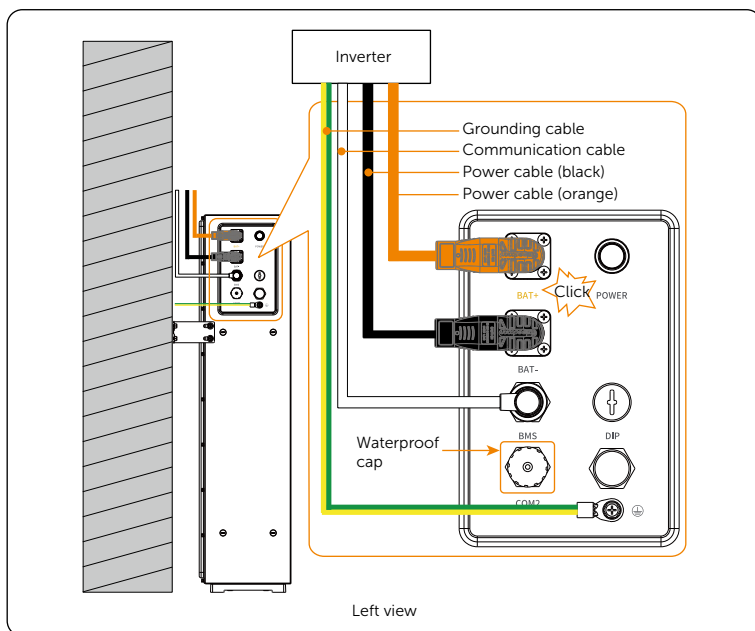
Figure 7-21 Cable connection of the left electrical connection area
