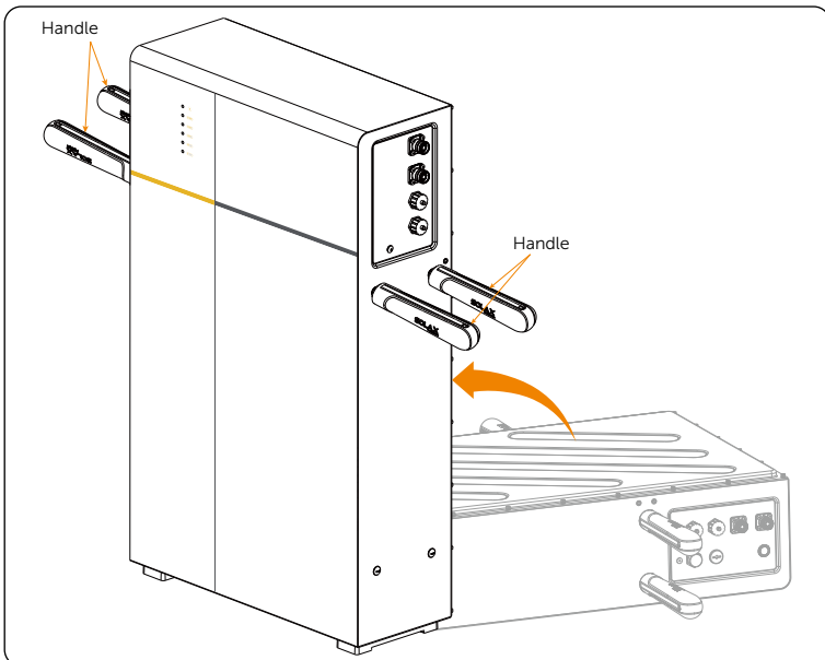
Figure 5-8 Lifting battery pack
