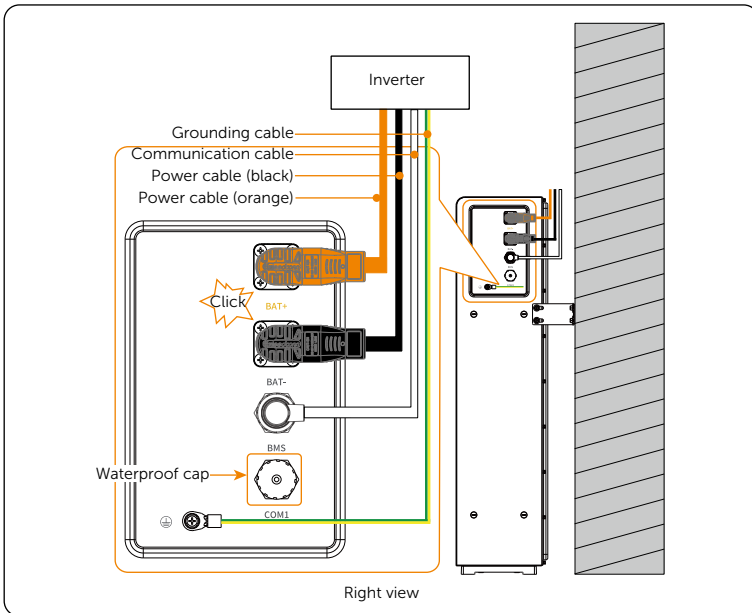
Figure 7-19 Cable connection of the right electrical connection area
