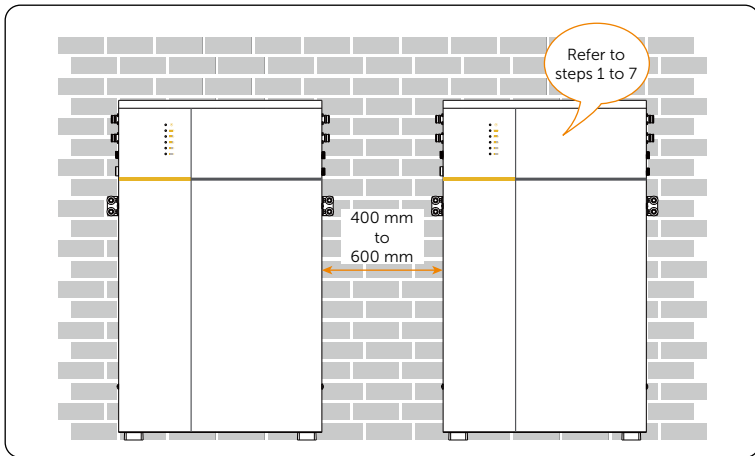
Figure 6-10 Installing the remaining battery pack
