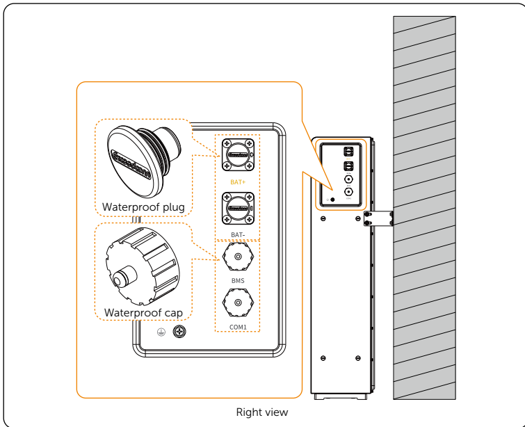
Figure 7-18 Right electrical area of the battery pack
