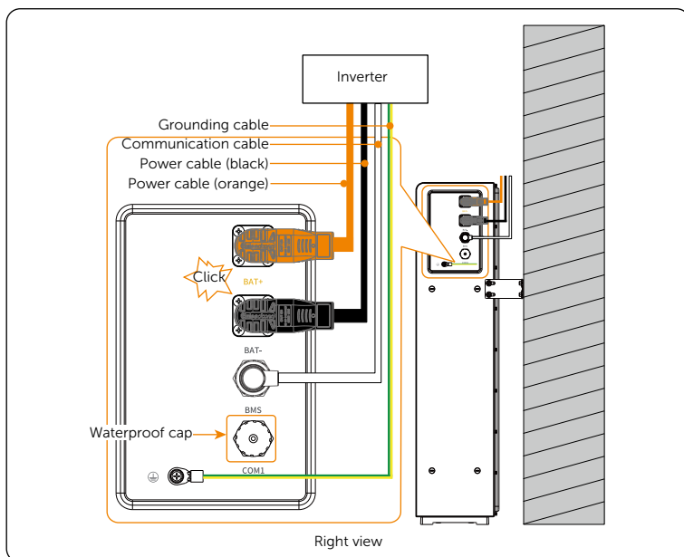
Figure 7-25 Cable connection of the right electrical connection area
