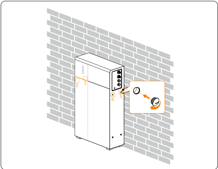
Figure 6-9 Inserting and tightening plastic plugs
