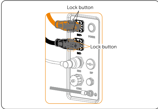
Figure 12-2 Unplugging power cables
