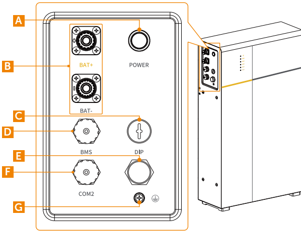
Figure 2-4 Left view
